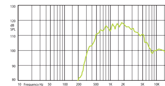
Frekvens respons
